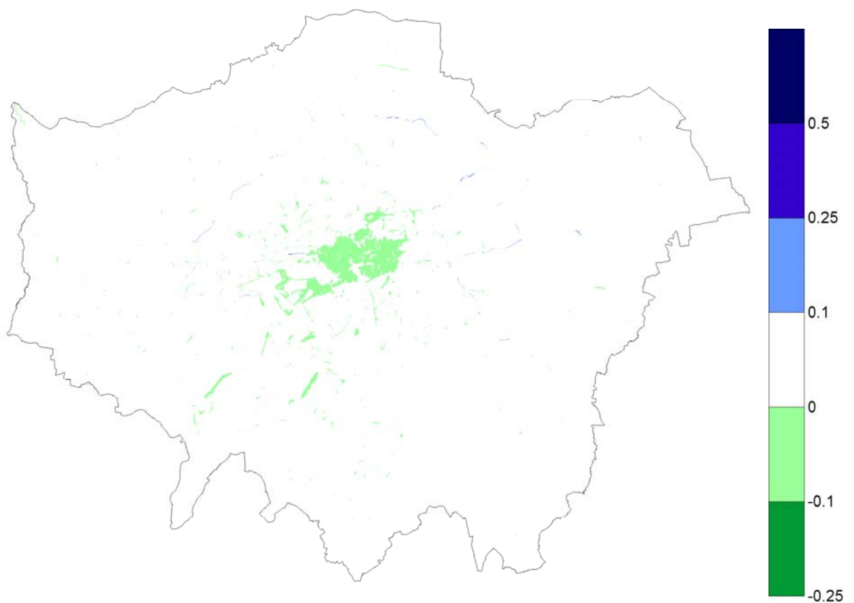
Postponement of LEZ: Predicted Impact on number of daily mean exceedences of PM10 in 2011.
