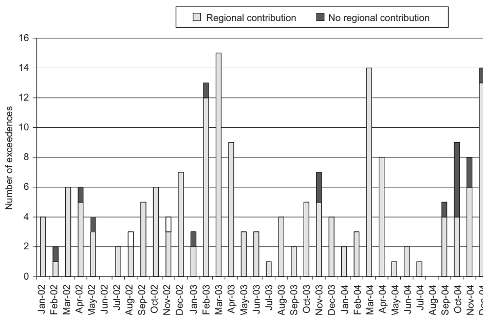
Fig. 3. Monthly number of exceedences of the PM_{10} limit value from January 2002 to December 2004. In grey, the number of exceedences with a contribution from the regional background and in black, the number of exceedences without a contribution from the regional background.
