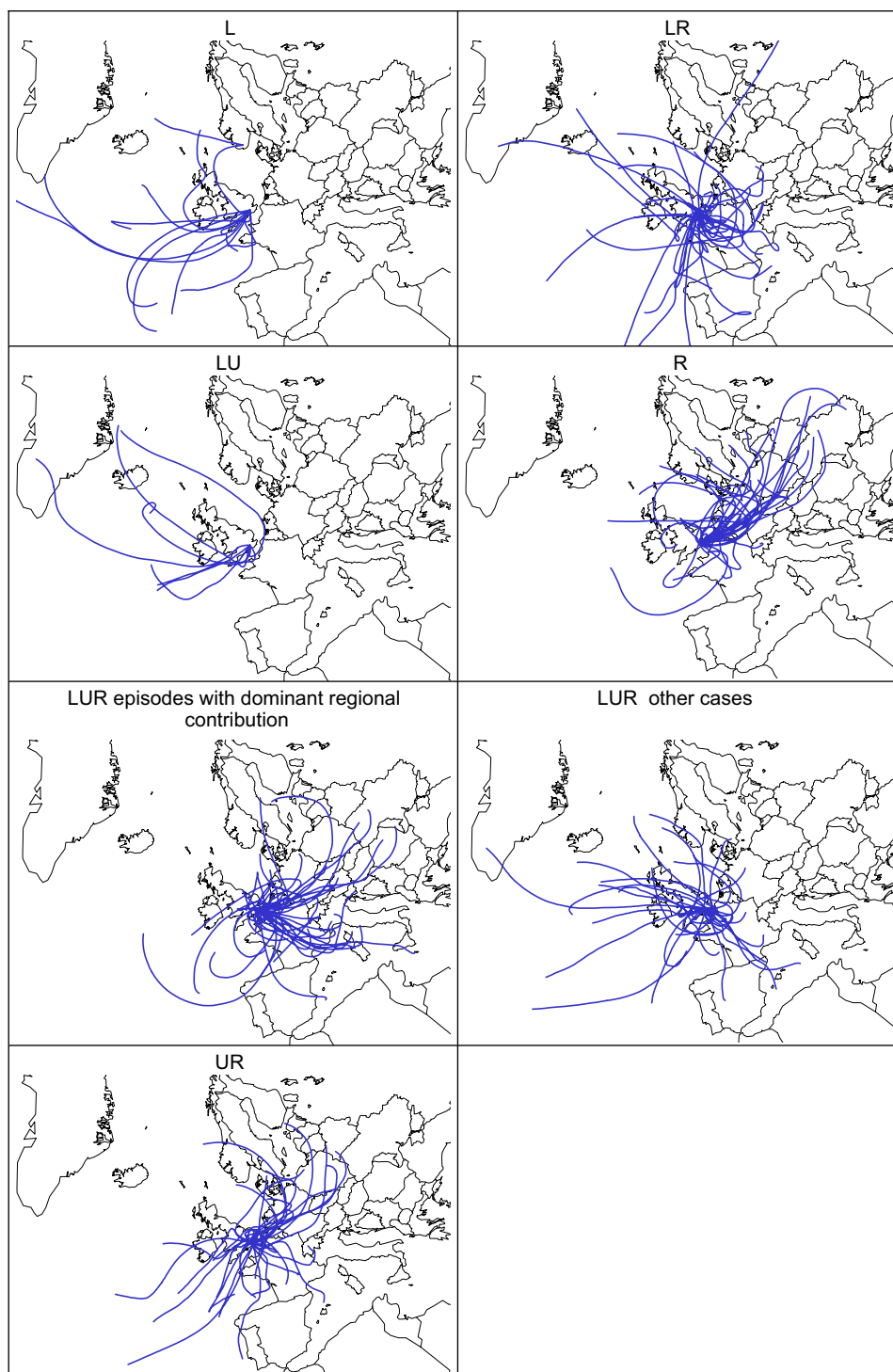
Fig. 4. Backward trajectories associated with each type of exceedance episode.
