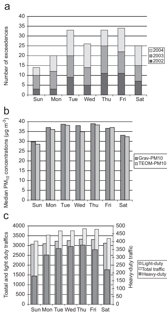
Fig. 2. (a) Number of exceedences of the PM 10 limit value as a function of the day of the week (2002–2004 data); (b) median daily gravimetric and TEOM PM 10 measured at Marylebone Road (2002–2004); (c) median numbers of light duty, heavy duty and total vehicles according to day of the week.
